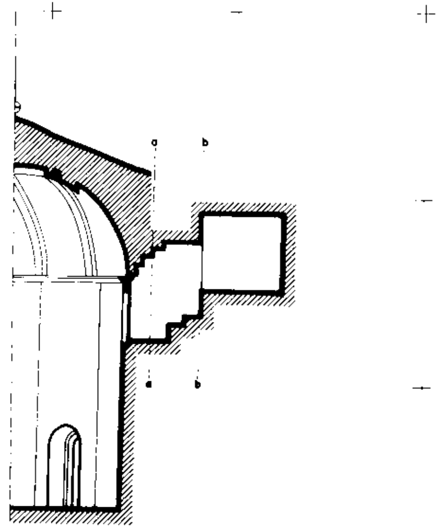
SECTION G-G
